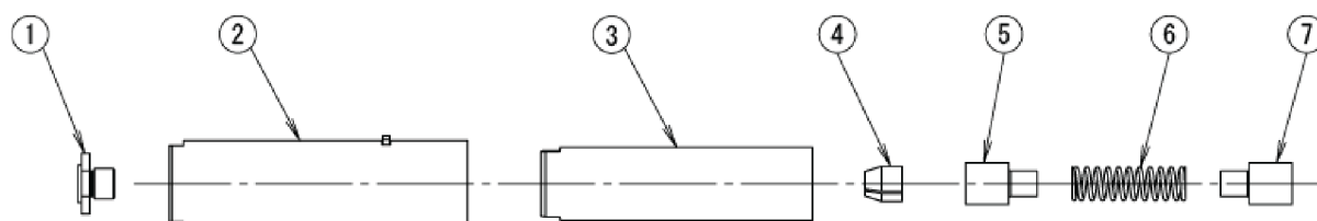
Fig. 5: Nose assembly AVSEAL 02964 14mm
