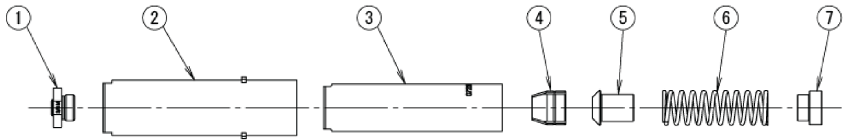
Fig. 3: Nose assembly
