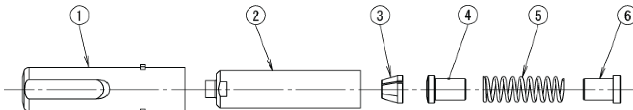
Fig. 2: Nose assembly
